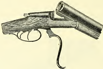
Daw's Hammerless Gun.
